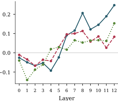
Phrase Role
